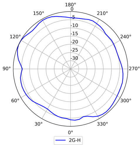
2.4G (Horizontal)
